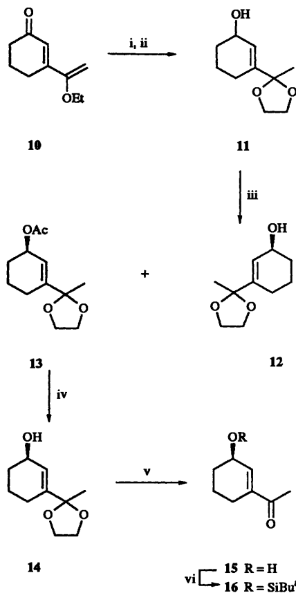
Scheme 2 Reagents and conditions: i, 2-ethyl-2-methyl-1,3-dioxolane, (\text{CH}_2\text{OH})_2 , CSA; ii, \text{NaBH}_4 , \text{CeCl}_3 \cdot 7\text{H}_2\text{O} , MeOH; iii, Lipase Amano AK, vinyl acetate, hexane; iv, \text{K}_2\text{CO}_3 , MeOH; v, \text{PTSA} \cdot \text{H}_2\text{O} , aq. acetone, reflux; vi, tert -butyldimethylsilyl chloride, DMAP, DMF
