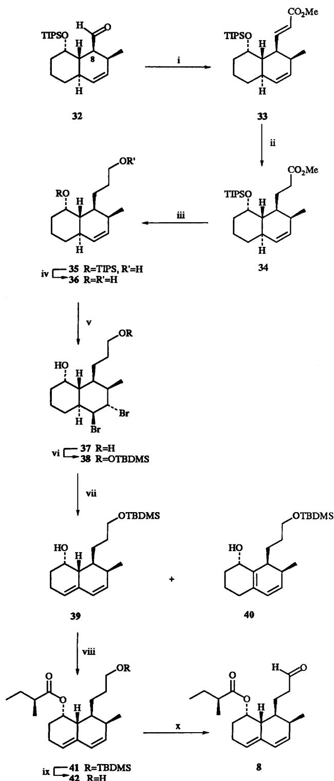
Scheme 6 Reagents and conditions: i, (\text{MeO})_2\text{P}(\text{O})\text{CH}_2\text{CO}_2\text{Me} , NaH, HMPA, THF, reflux; ii, Mg, MeOH, 0 °C; iii, LAH, ether; iv, aq. HF acetonitrile; v, \text{Br}_2 , \text{CH}_2\text{Cl}_2 ; vi, TBDMSOTf, 2,6-dimethylpyridine, \text{CH}_2\text{Cl}_2 ; vii, DBU, HMPA, 60 °C; viii, ( S )-2-methylbutanoic anhydride, DMAP, \text{CH}_2\text{Cl}_2 ; ix, TBAF, THF; x, (\text{COCl})_2 , DMSO, \text{Et}_3\text{N} , \text{CH}_2\text{Cl}_2
