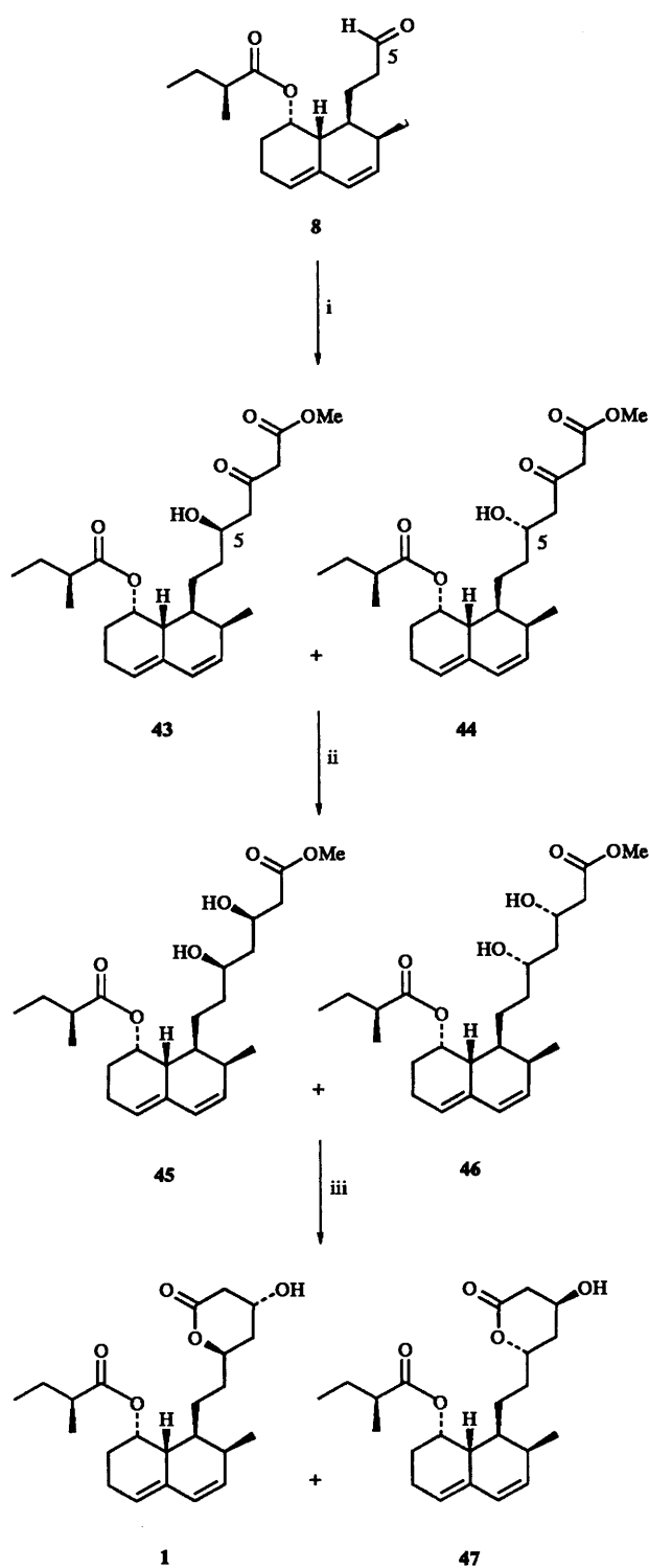
Scheme 7 Reagents and conditions: i, BuLi, NaH, 9, THF, 0 °C or \text{TiCl}_2(\text{OPr}^i)_2 , bistrimethylsilyl enol ether 9, \text{CH}_2\text{Cl}_2 , -78 °C; ii, \text{Et}_2\text{BOMe} , \text{NaBH}_4 , MeOH, -78 °C; iii, HF-pyridine complex, acetonitrile
